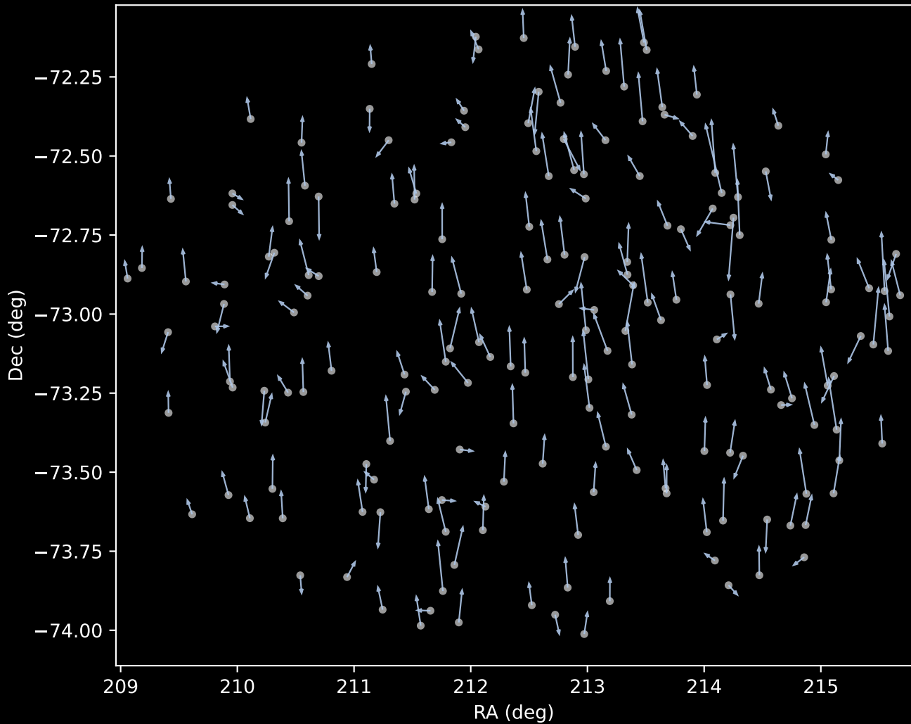
GALAH DR4 Cluster 1 Proper Motion Vectors (n=187)
