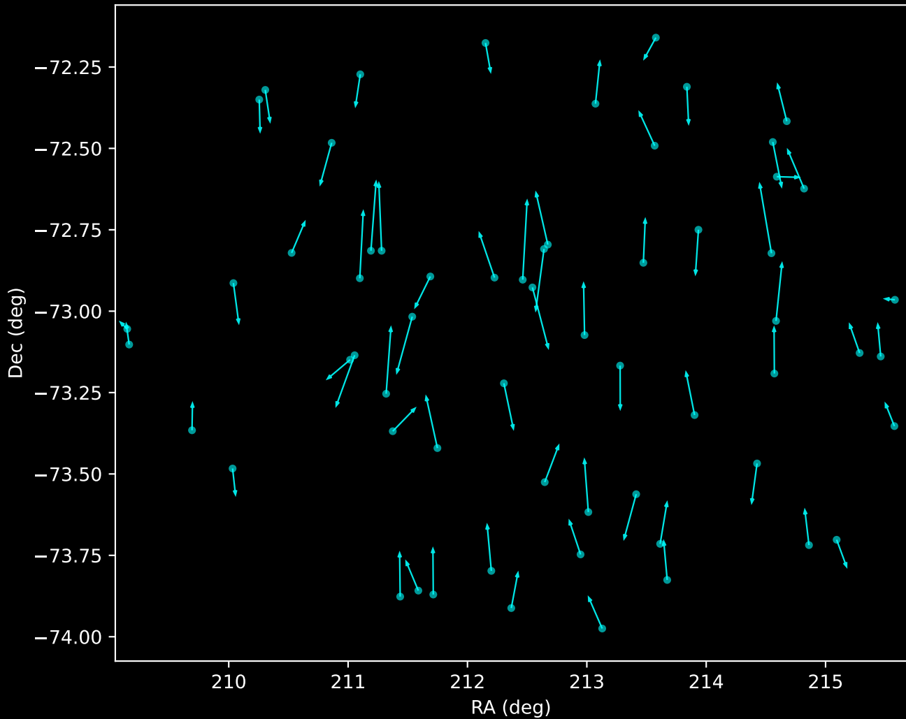
GALAH DR4 Noise Stream Proper Motion Vectors (n=62)
